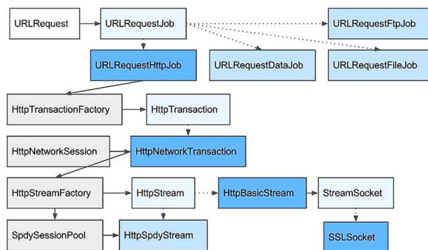
Fig. 2 Network stack of a Chromium WebView [21]
