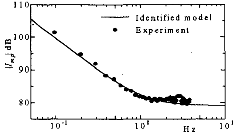
Fig. 7. Identification of impedance characteristic
