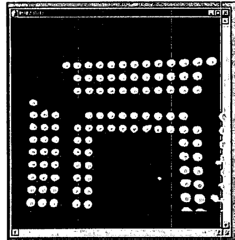
Fig.6 Binary image data (minus 37 degrees).
