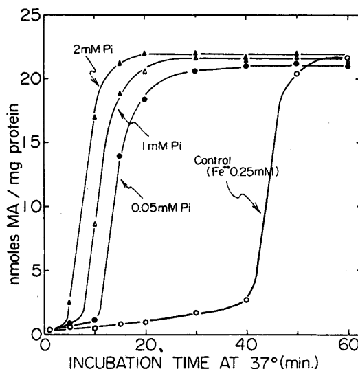
Fig. 1. Effect of inorganic phosphate (Pi) on the lipid peroxidation of rat liver mitochondria induced by \text{Fe}^{++} in KT (0.15M KCl, 0.01M, Tris-Cl, pH 7.4)-medium at 37°. Pi concentration in the medium is given in figure and reaction was started by addition of \text{Fe}^{++} (0.25mM).
