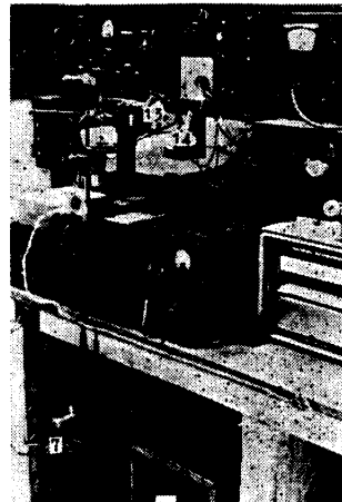
Fig. 2 Photographs of the apparatus. 1: tungsten lamp, 2: prism monochromator, 3: half mirror, 4: photomultiplier 1P 22, 5: D. C. amplifier, 6: autorecorder, 7: stabilizer, 8: source of mercury lamp, 9: mercury lamp, 10: grating mirror monochromator, 11: photomultiplier 1P 21, 12: rotating platinum electrode, 13: synchronous motor, 14: calomel half cell, 15: oxymeter, 16: sample room, 17: water bath.
