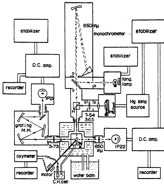
Fig. 1 Outline of the apparatus. tang. lamp: tungsten lamp, monochromator: prism monochromator, H: half mirror, 650 mμ: 650 mμ filter, 1P 22: photomultiplier, D. C. amp.: D. C. amplifier, recorder: autorecorder, stabilizer: stabilizer, Hg lamp source: source of mercury lamp, Hg: mercury lamp, 7-54: filter of Corning No 9863, 365: Hitachi filter 365 mμ, 3-73: filter of Corning No 3389, grating M. M.: grating mirror monochromator, 1P 21: photomultiplier, Pt: rotating platinum electrode, motor: synchronous motor, C. H. cell: calomel half cell, oxymeter: oxymeter constructed by the method of Hagihara 1 , water bath: water bath, D: diaphragm.
