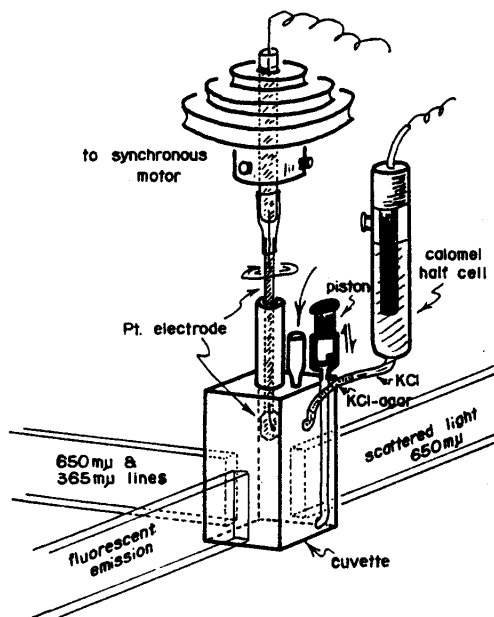
Fig. 3 Diagram of a sample cuvette for polarographic, 90° light-scattering and fluorometric analysis.
