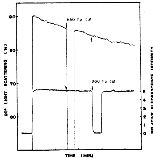
Fig. 5 Effects of excitation light at 365 m\mu and fluorescent emission on 90° light scattering at 650 m\mu and of the 650 m\mu line for light scattering on the fluorescent emission at 450 m\mu .
