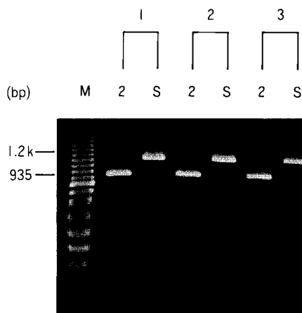
Fig. 6 Haptoglobin (Hp) genotyping from three bloodstains of Hp^2 - Hp^{1S} stored at room temperature for three years.
