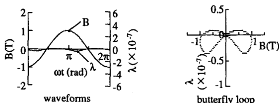
Fig.10 Waveforms of flux density B and magnetostriction \lambda and butterfly loop for low magnetostriction 6.5% silicon steel (thickness : 0.35mm, B_m=1.0\text{T} , 50Hz).
