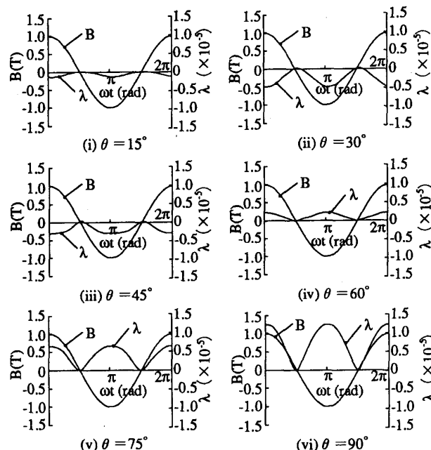
Fig.11 Waveforms of flux density and magnetostriction in various direction \theta for highly-oriented silicon steel (M-0H, thickness : 0.3mm, B_m=1.0\text{T} , 50Hz).
