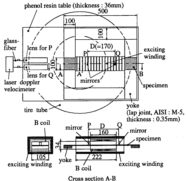
Fig.2 Experimental equipment.
