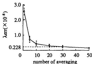
Fig.9 Effect of averaging ( D=170\text{mm} ).
