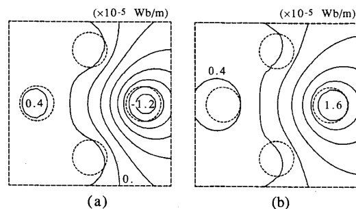
Fig.5 Equipotential lines for four wire model with J_A = -\sigma \exp(j\omega t) , J_B = J_C = J_D = 0 , (a) real part, (b) imaginary part.
